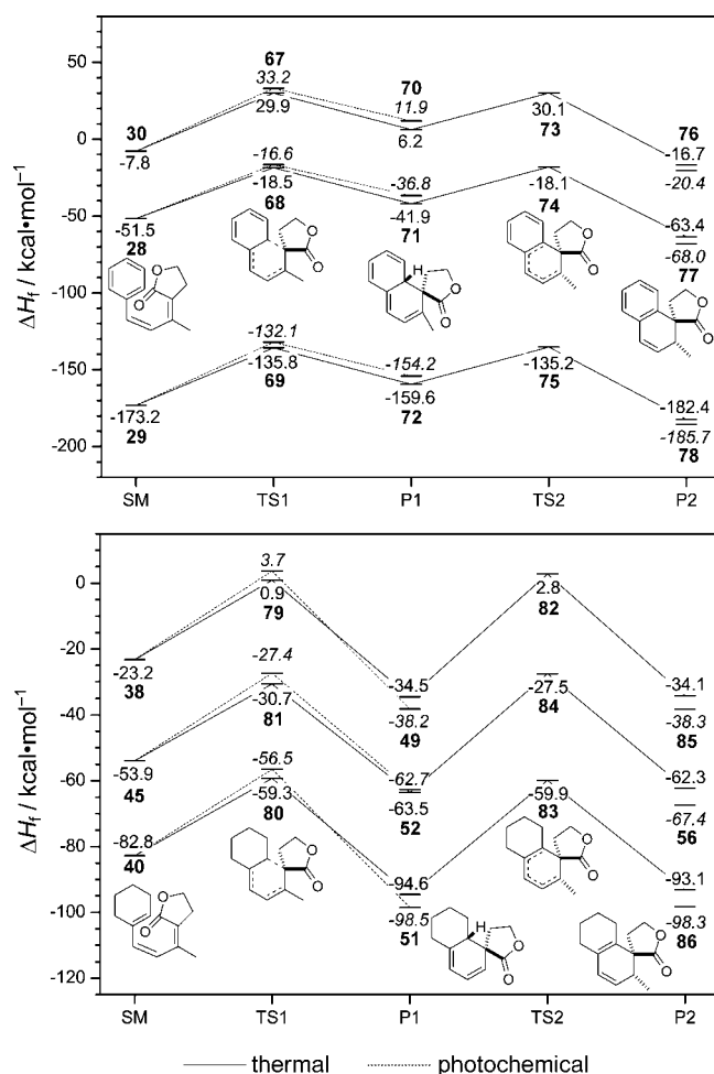
Figure 3. Calculated energy profiles for the cyclisation reactions of compounds 28–30 (top) and for the saturated series 38 , 40 , and 45 (bottom). Enthalpy values in italics refer to the photochemical pathway.
